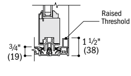
On-Floor Drainage Sill Optional Raised Threshold
