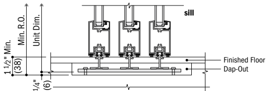
Vertical Section Flush Sill
