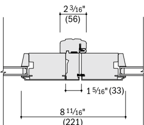
Horizontal Section Astragal, Passive Panel-Active Panel
