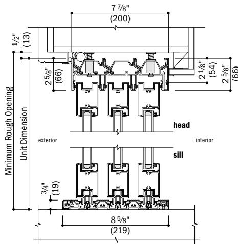
Vertical Section On-Floor Drainage Sill Three-Panel, One-Direction Panel Operation
